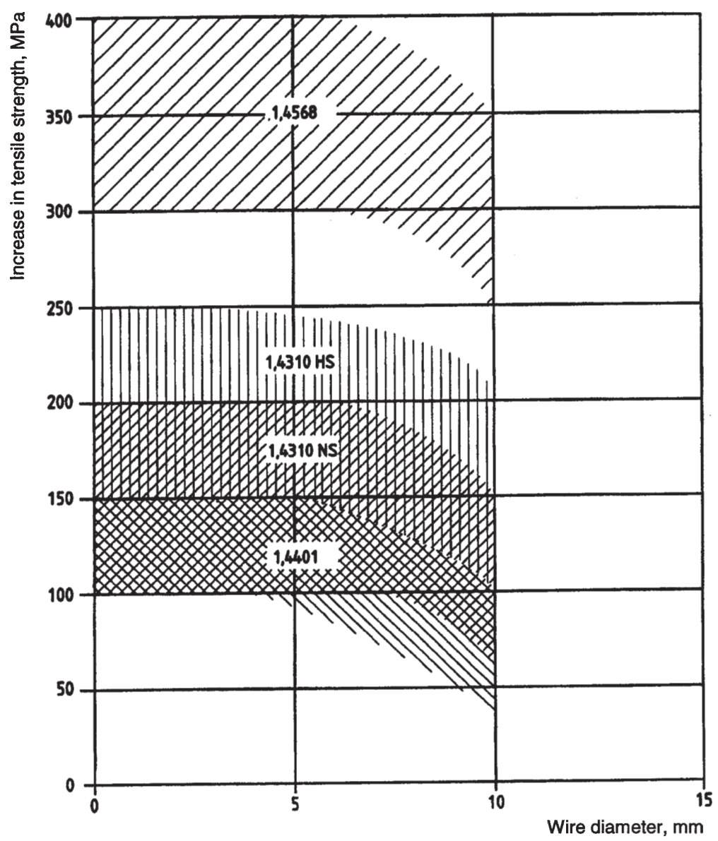
Figure A.1 — Reference data for the increase in tensile strength of cold drawn wire by heat treatment (see Table A.2)
